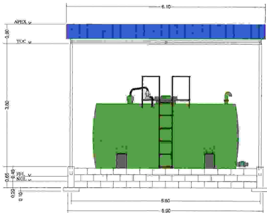
○ FRONT / REAR ELEVATION
