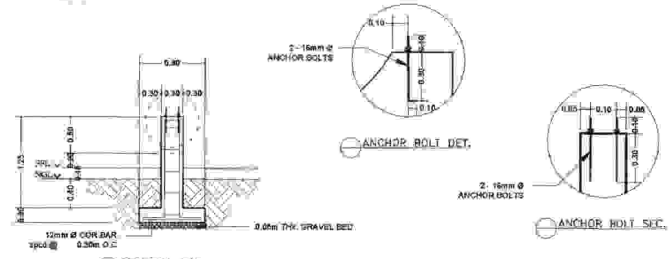
PEDESTAL SEC.
