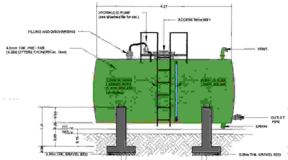
CYLINDRICAL TANK DET.
