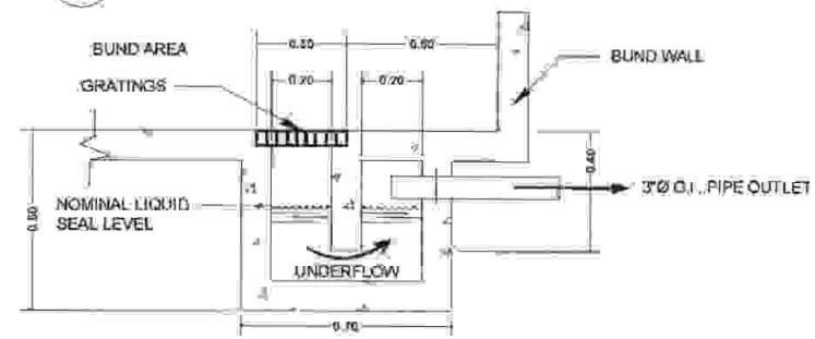
OIL & STORM WATER TRAP SECTION DET.
