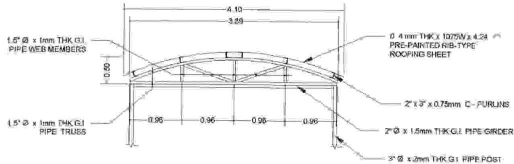
ROOF DETAIL
