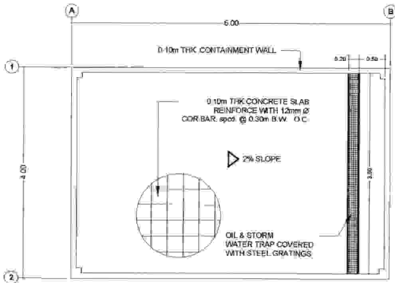
SECONDARY CONTAINMENT PLAN
