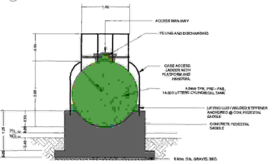
PEDESTAL SEC.
