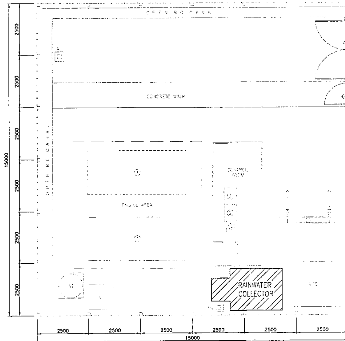
SITE DEVELOPMENT PLAN SCALE 1:75
